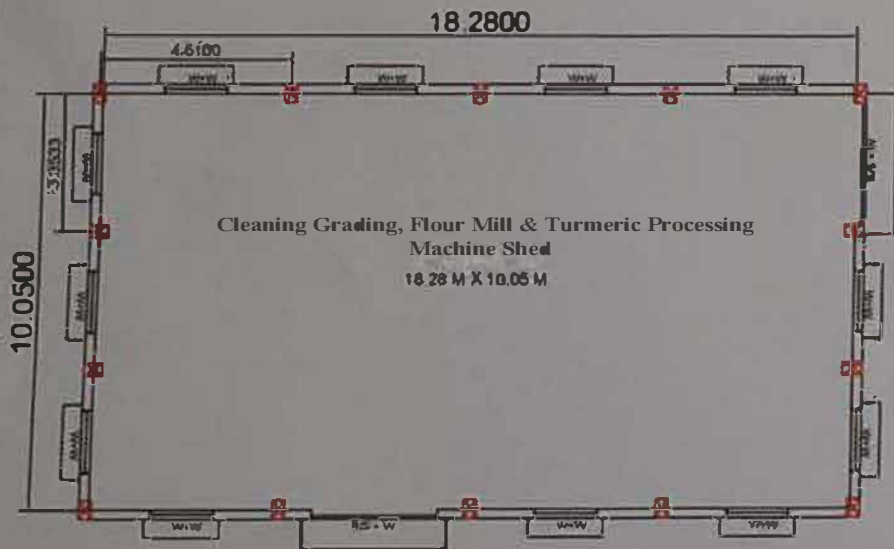
C&G, Flour Mill & Turmeric Processing Machine Shed scale 1:100
